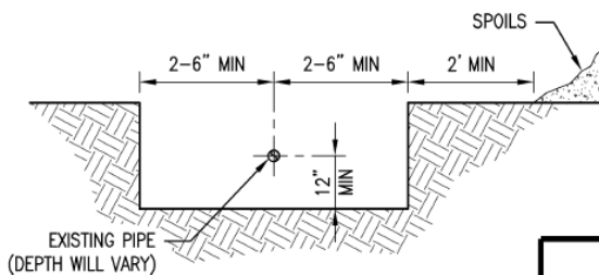
BELLHOLE DETAIL ELEVATION VIEW
