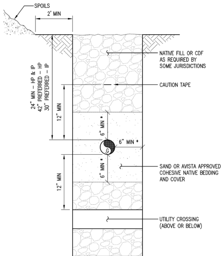
GAS MAIN TRENCH DETAIL
