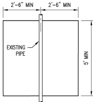
BELLHOLE DETAIL PLAN VIEW
