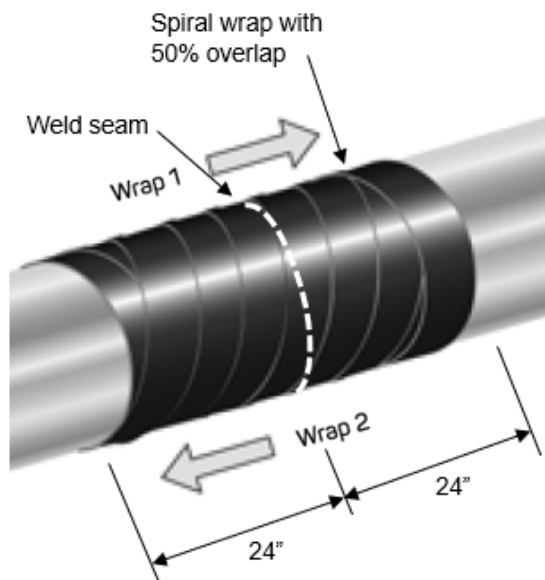
Optional 4-layer application
