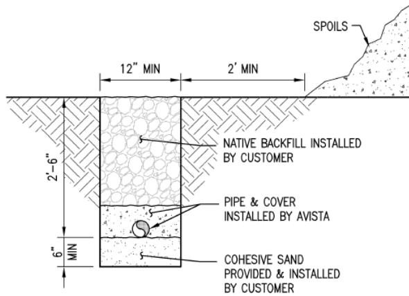
TRENCH DETAIL ELEVATION VIEW
