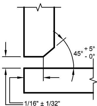
JOINT DESIGN (BRANCH)
