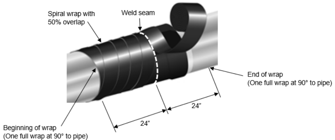
Standard 2-layer application
