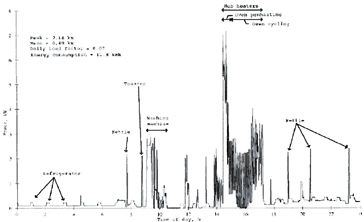
Figure 1: Household Electricity Demand Profile Recorded on a One-minute Time Base 5
